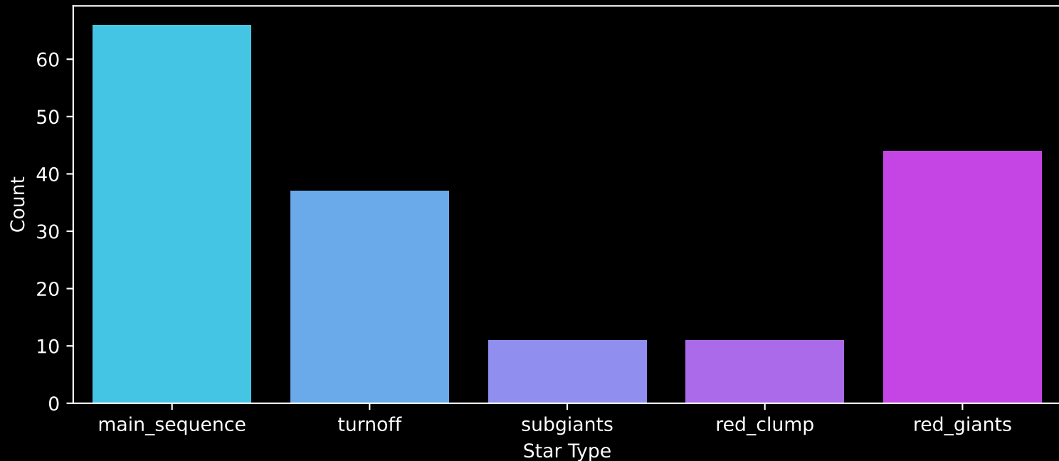
APOGEE DR17 Field: [INTCL_N7078_MGA] Count plot of Star Type
