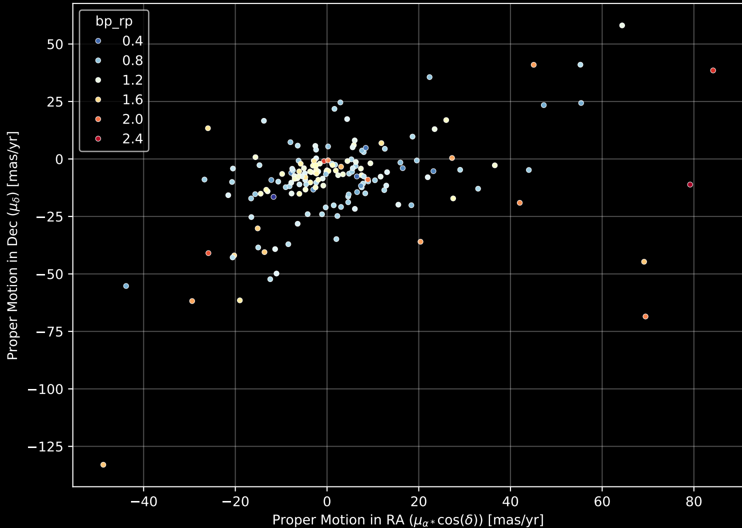
APOGEE DR17 Field: [INTCL_N7078_MGA] Proper Motion Diagram (n= 169)
