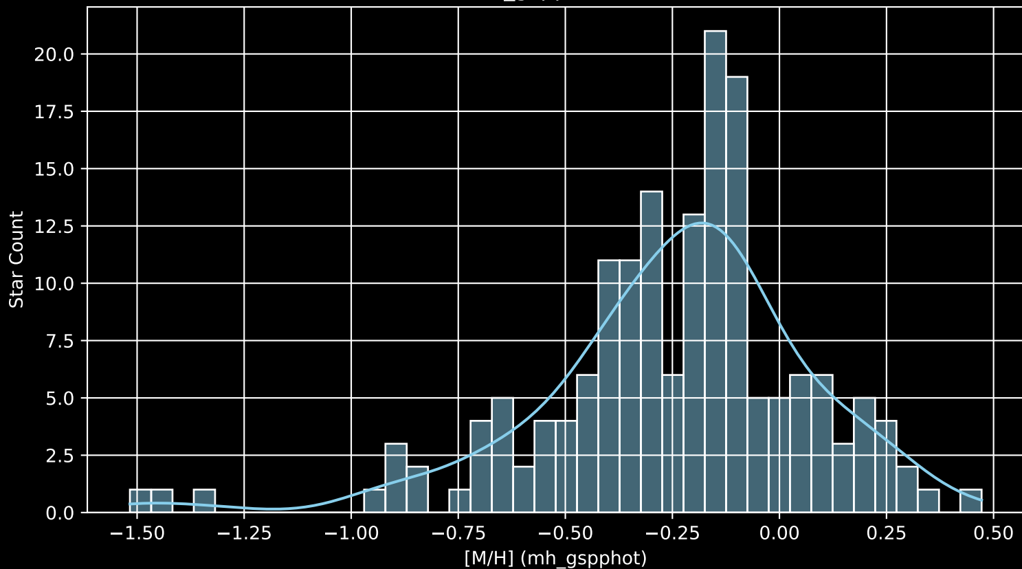
APOGEE DR17 Field: [INTCL_N7078_MGA [M/H] (mh_gspphot) (n= 168)
