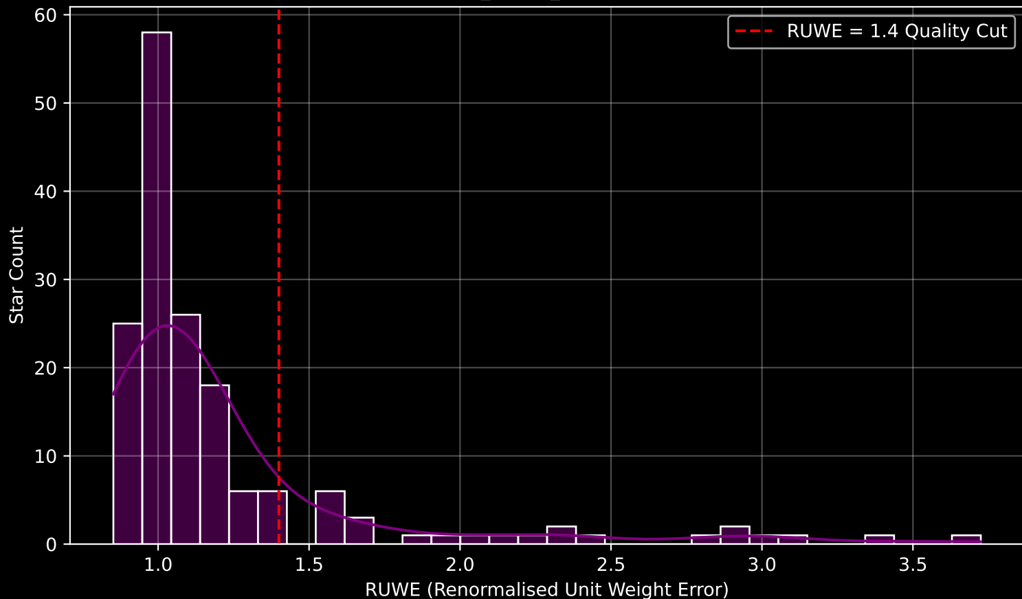
GAPOGEE DR17 Field [INTCL_N7078_MGA] RUWE Distribution (n= 163)
