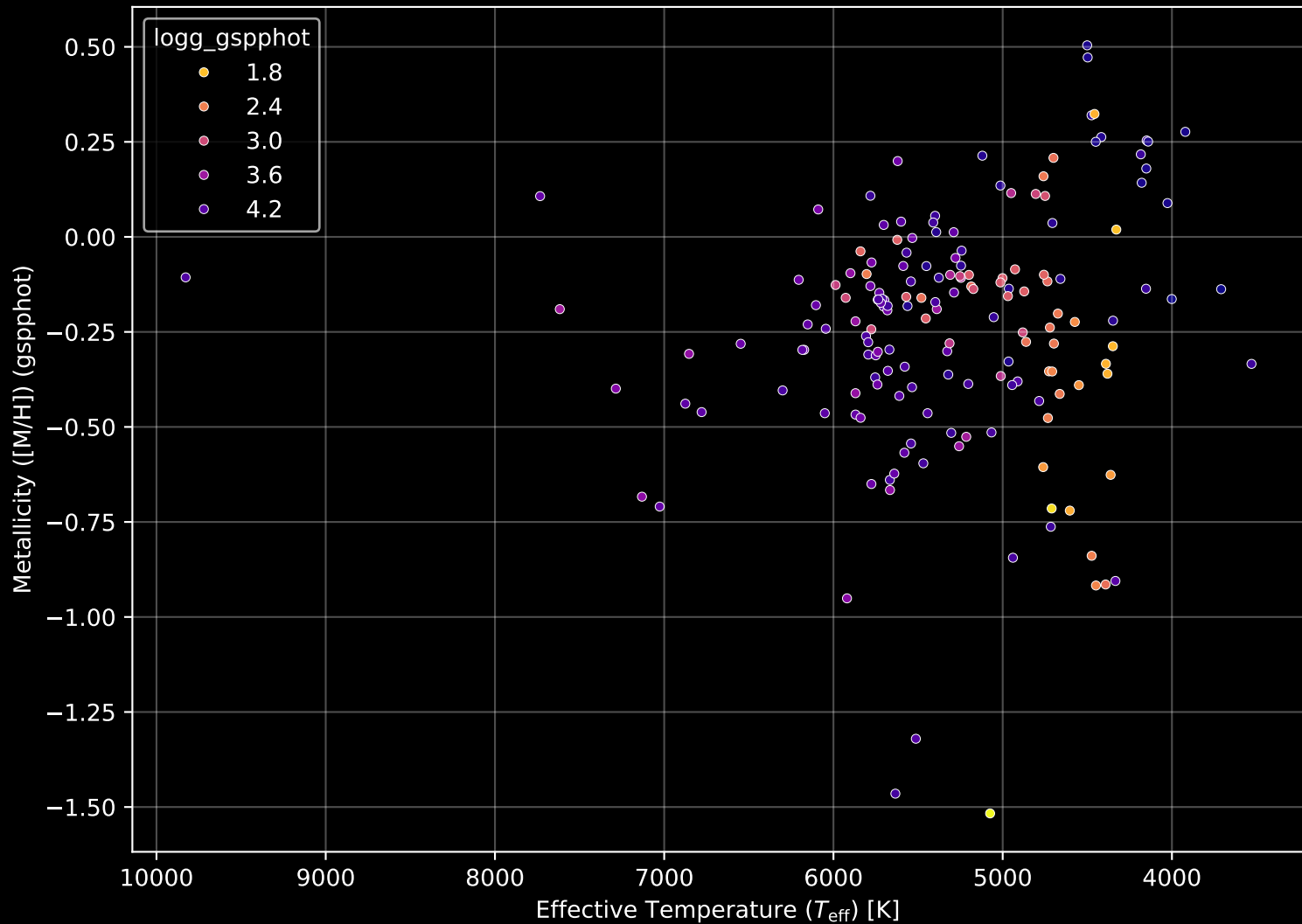
APOGEE DR17 Field: [INTCL_N7078_MGA] Stellar Population Parameters (n= 169)
