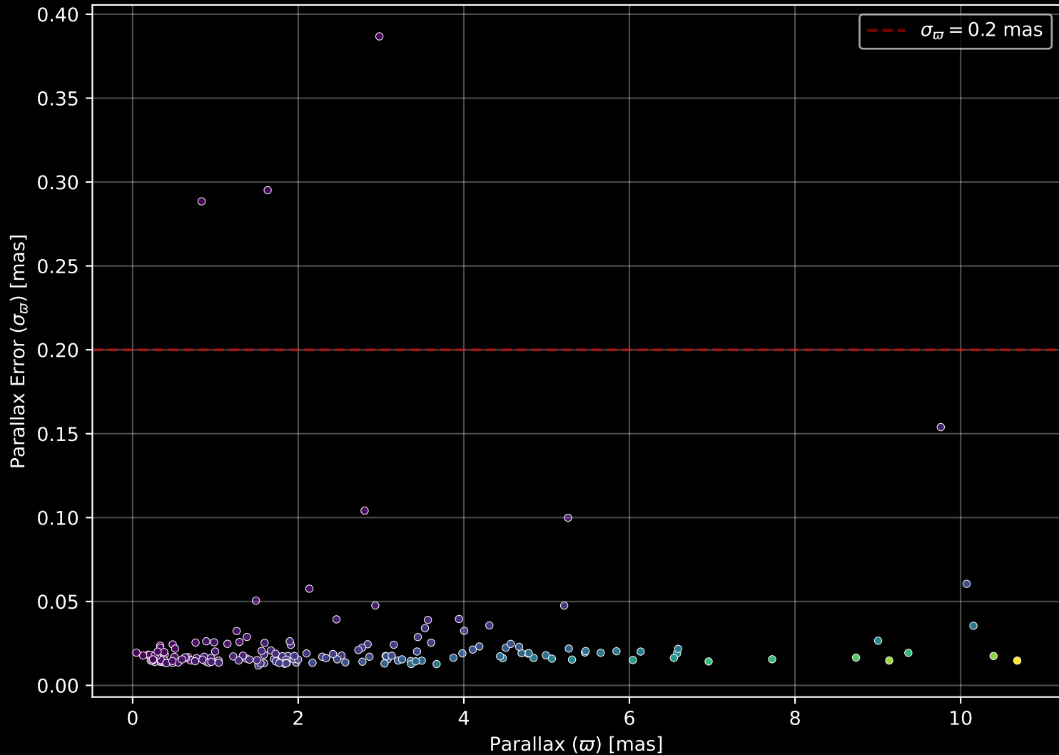
APOGEE DR17 Field: [INTCL_N7078_MGA] Parallax Quality (n= 169)
